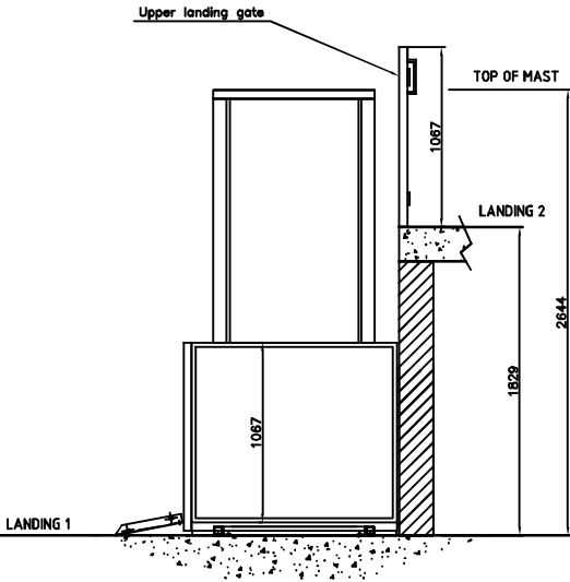
Side view for Elevex Typ 2
