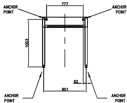
4 Anchor points
