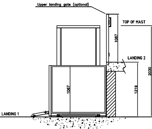
Side view for Elevex Typ 1
